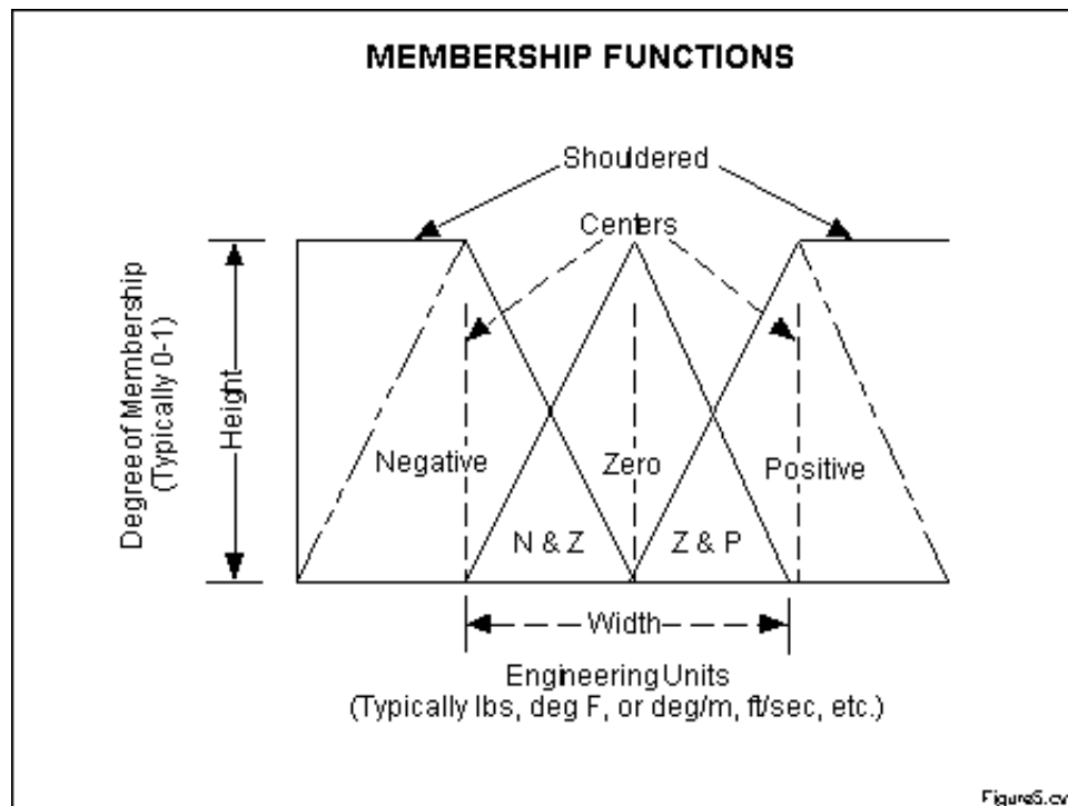
Figure 5 - The features of a membership function
