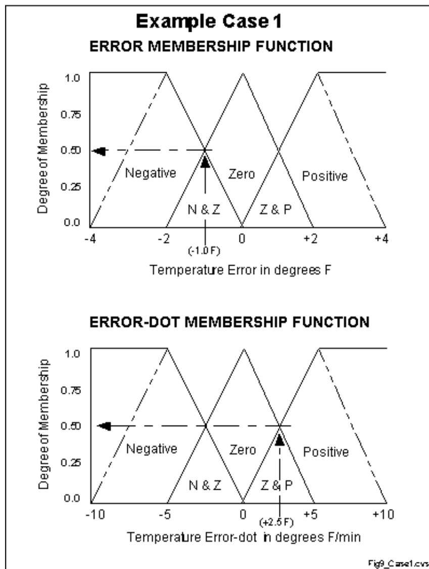
Figure 9 - EXAMPLE CASE 1: (initial conditions)
