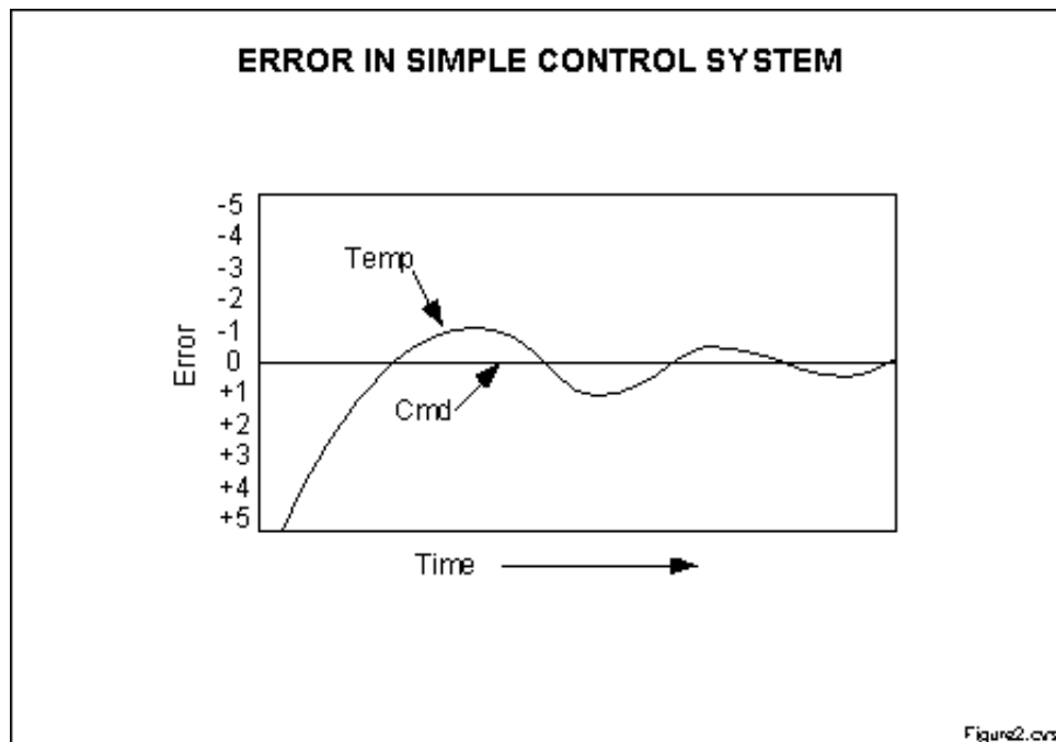
Figure 2 - Typical control system response
