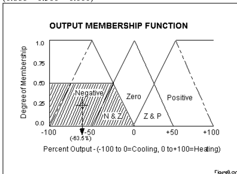
Figure 8 - The horizontal coordinate of the centeroid is taken as the crisp output
